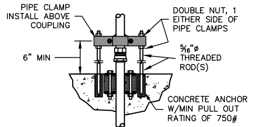
PIPE CLAMP (FLOOR) NTS
