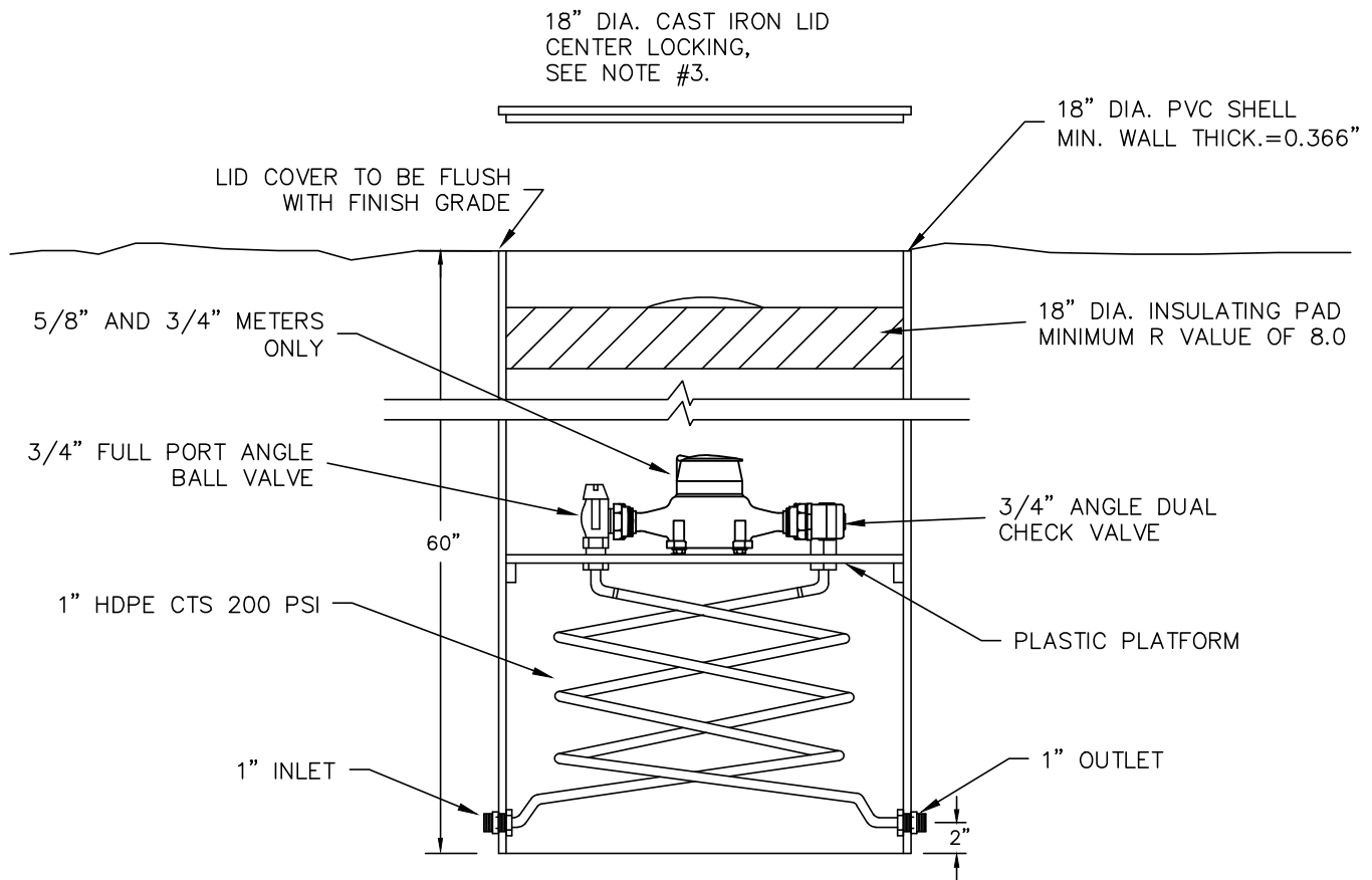
ELEVATION VIEW
